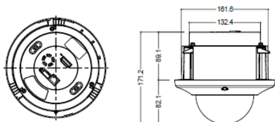
Indoor In-ceiling(PSF-M108)
