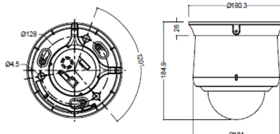
Indoor Surface(PS-M108)
